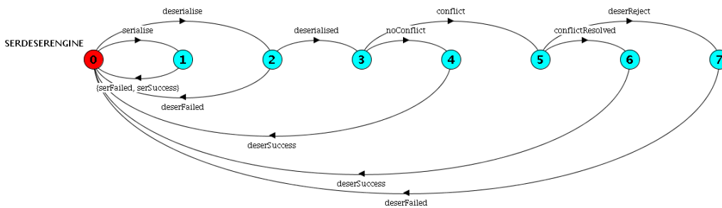
Figure 3.7: A state machine representing the Serialisation & Deserialisation Engine.
